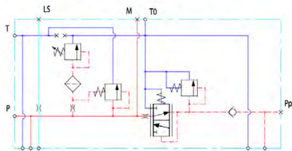
Closed center PVP with PPRV and T0
