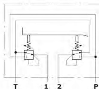
SVM500 Hydraulic circuit
