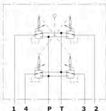
Hydraulic circuit
